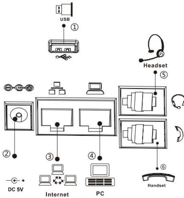
Picture 3 - Connecting to the Device
