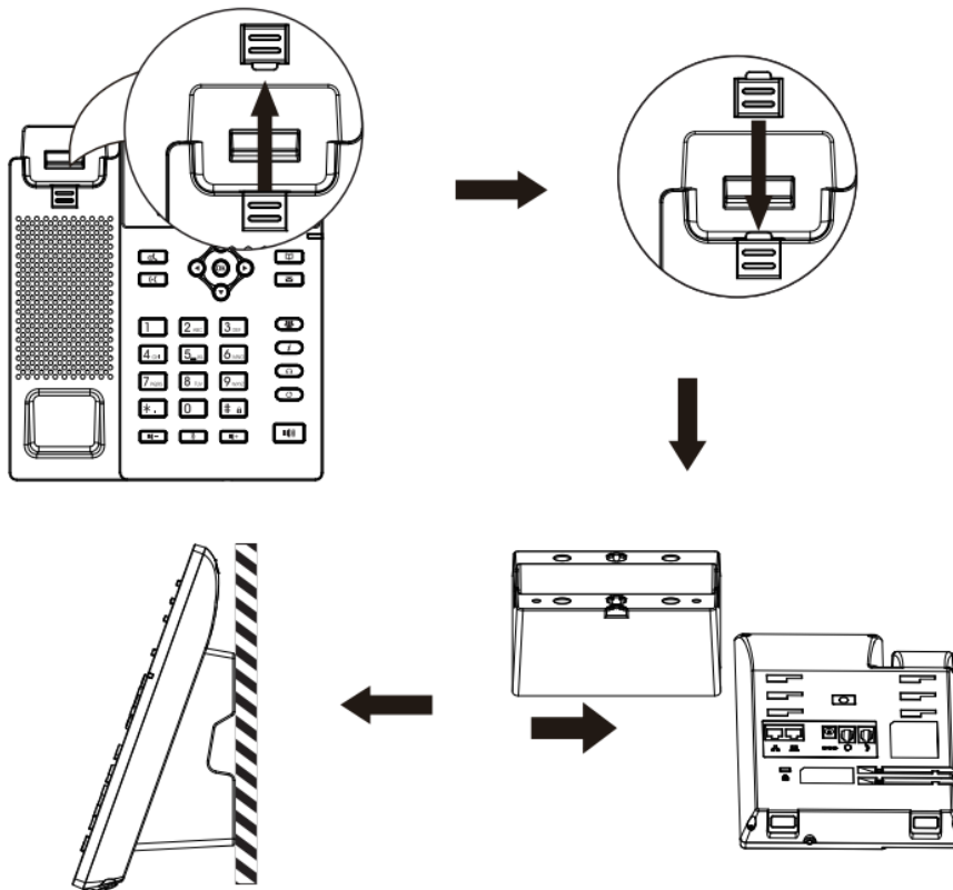
Picture 2 - Wall-mounted installation
